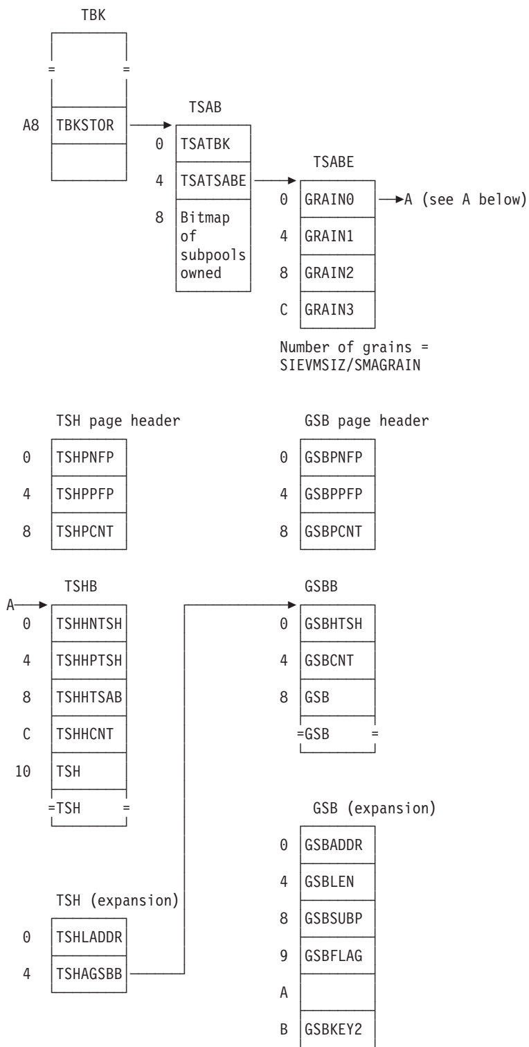
Figure 11. TSHB and GSBB Control Blocks
